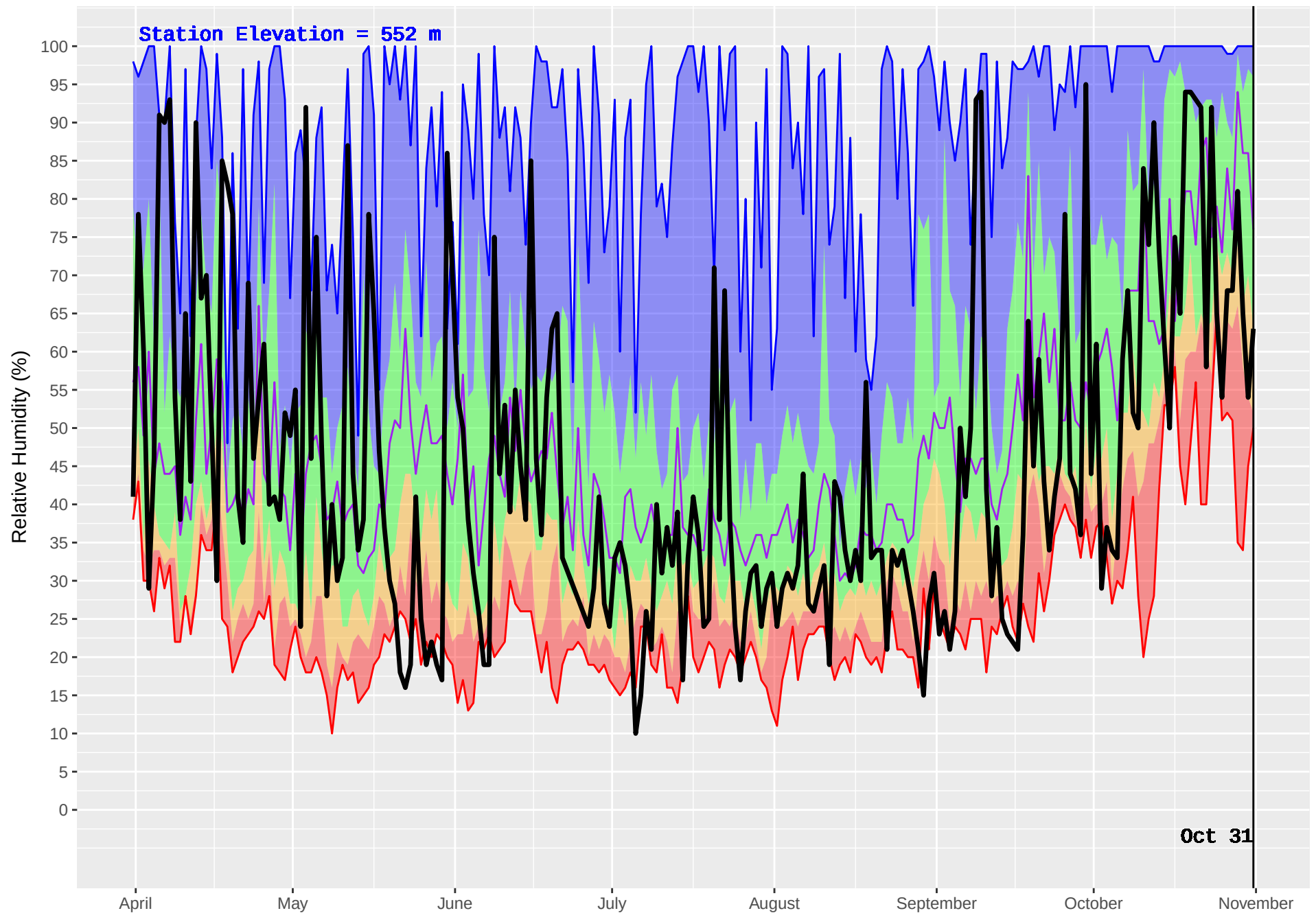
NAHATLATCH (316) : Historical (2001–2016) and Current (2017) Noon Relative Humidity
