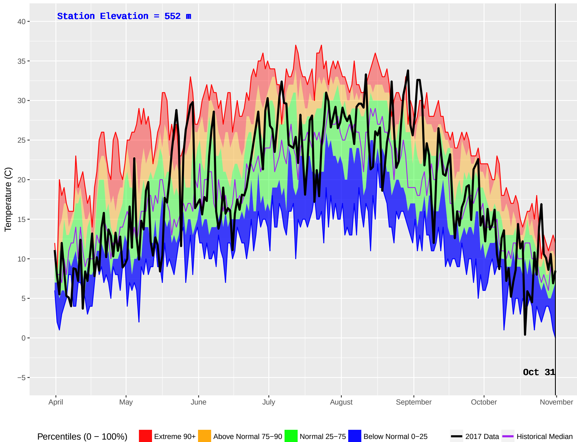
NAHATLATCH (316) : Historical (2001–2016) and Current (2017) Noon Temperature
