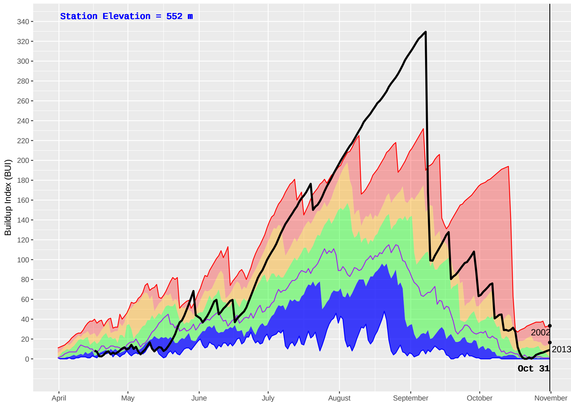
NAHATLATCH (316) : Historical (2001–2016) and Current (2017) Noon Buildup Index (BUI)
