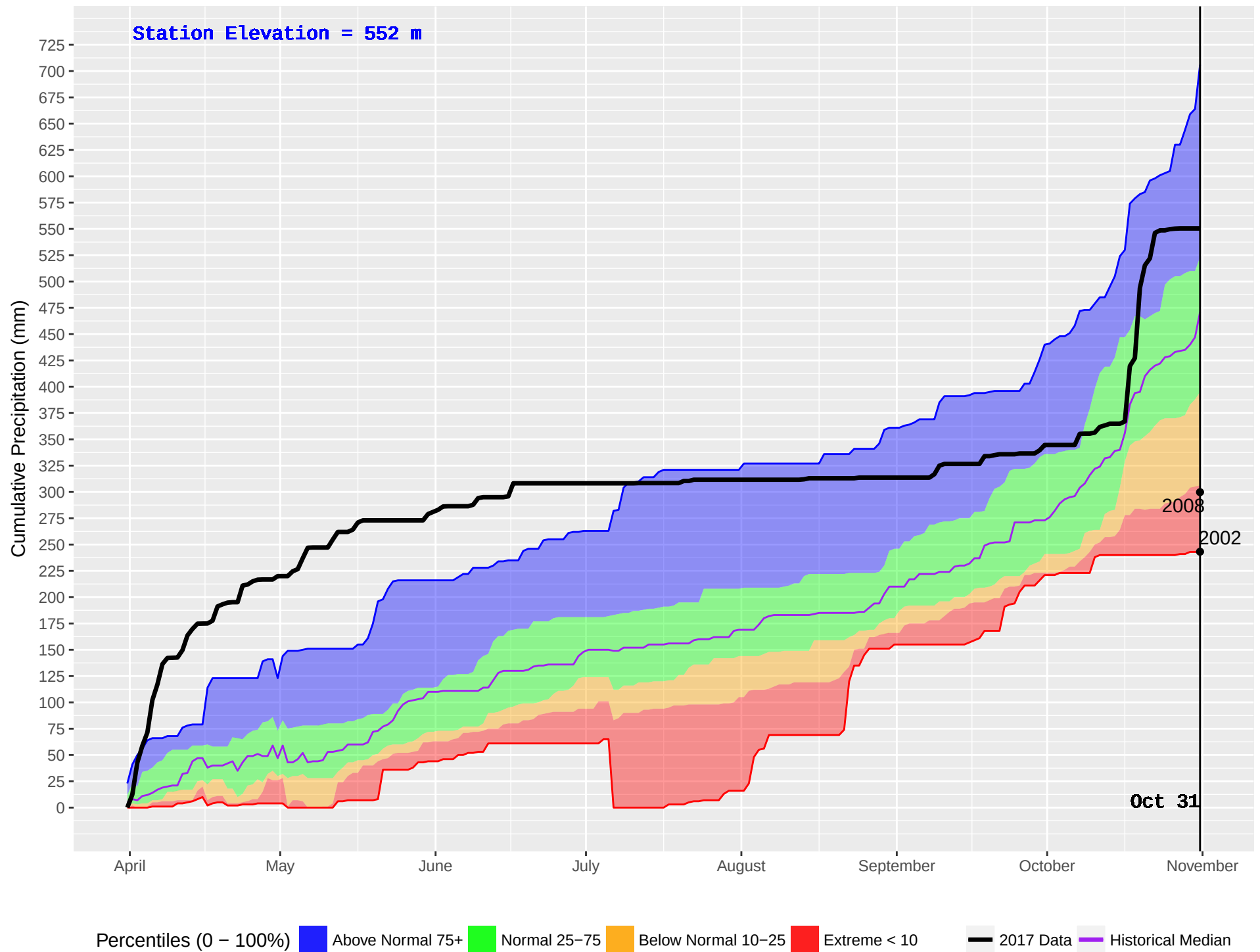
NAHATLATCH (316) : Historical (2001–2016) and Current (2017) Noon Cumulative Precipitation
