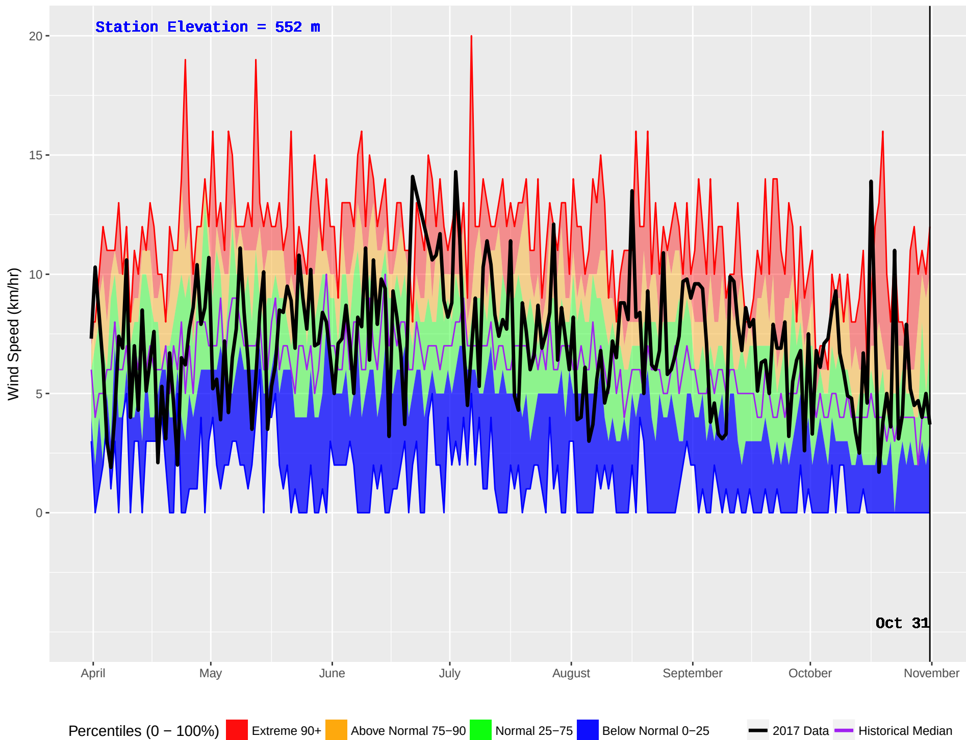
NAHATLATCH (316) : Historical (2001–2016) and Current (2017) Noon Wind Speed
