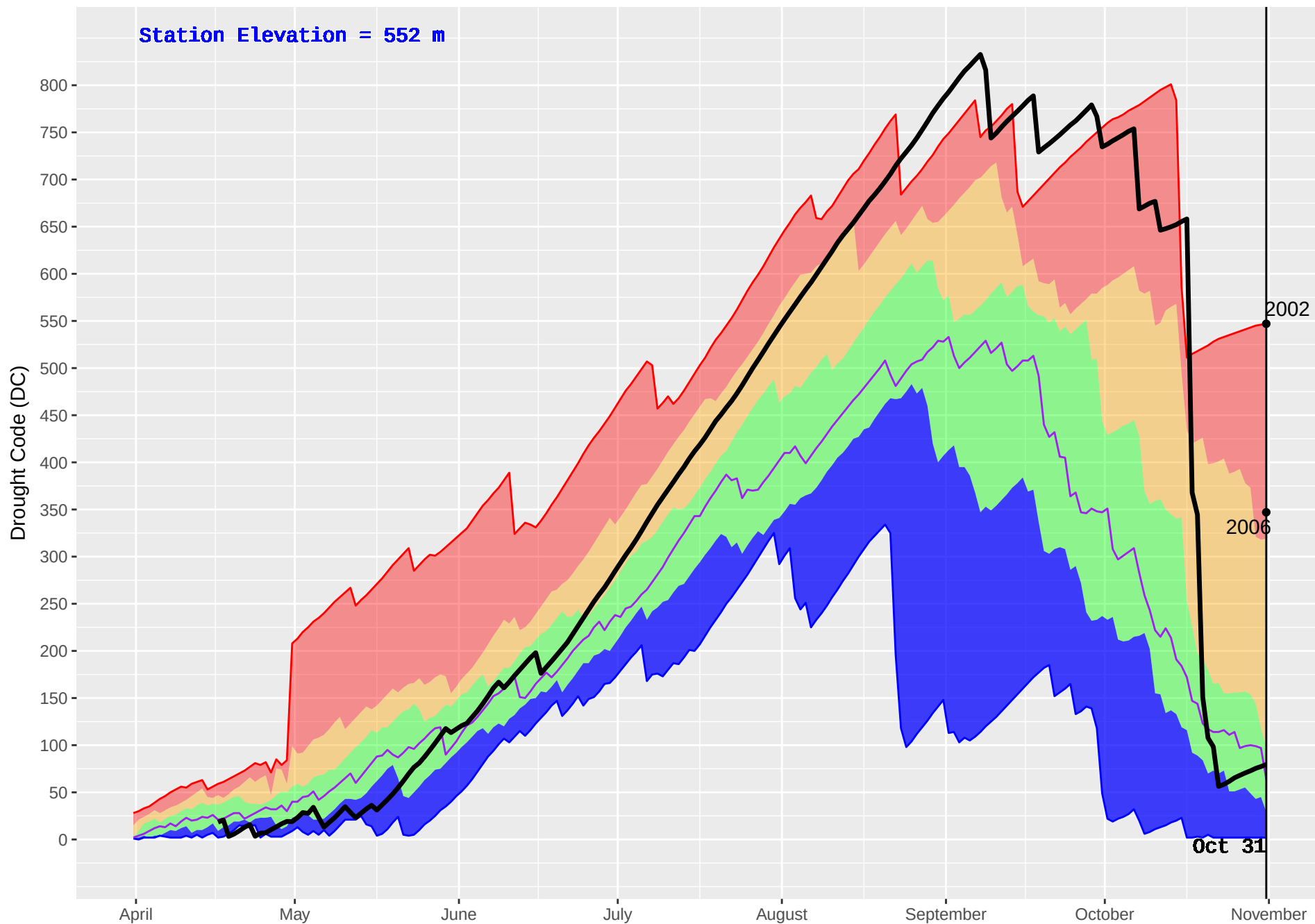
NAHATLATCH (316) : Historical (2001–2016) and Current (2017) Noon Drought Code (DC)
